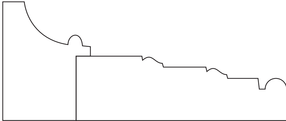
BA 1794 1-1/4" x 3-11/16"
