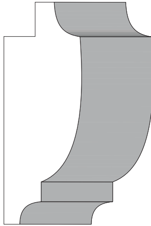
BA 1752 13/16" x 2-5/16"
