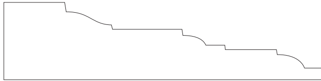
BA 1737 13/16" x 3-1/2"
