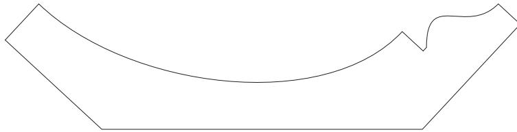
BA 1687 1" x 3-15/16"
