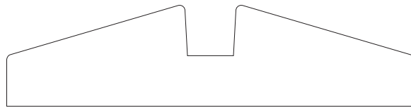
BA 1593 3/4" x 3"
