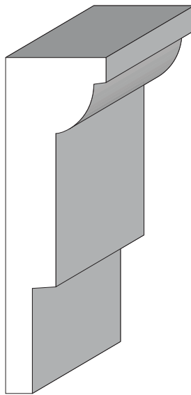
BA 1591 3/4" x 2-1/2"
