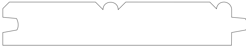
BA 1386 3/4" x 4-1/4"
