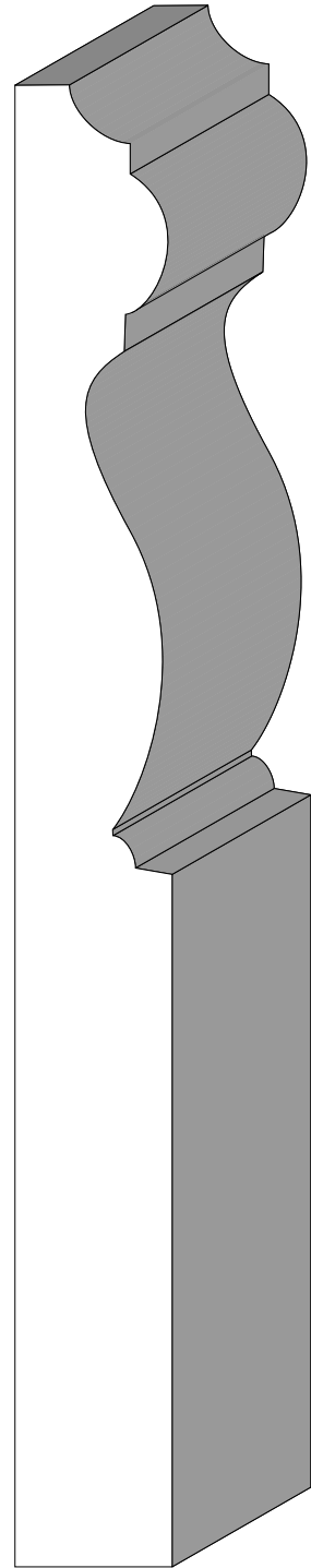
BA 1369 3/4" x 7-1/16"
