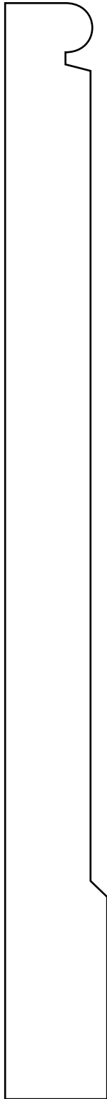
BA 1340 3/4" x 8"
