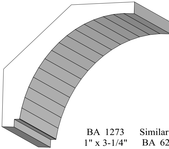
BA 1273 1" x 3-1/4"
