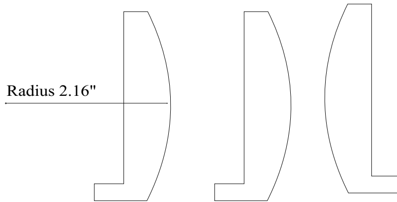
BA 1140 13/16" x 2"
