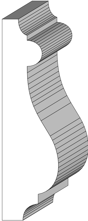
BA 1074 1-3/16" x 4-1/4"
