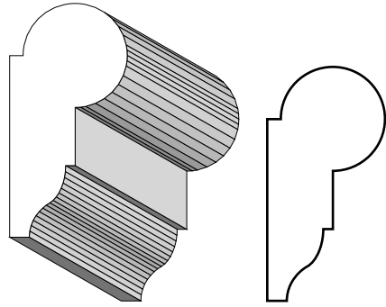
BA 913 3/4" x 1-3/8"
