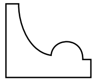
BA 879 3/4" x 7/8"
