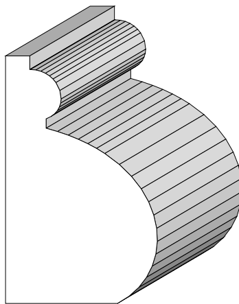
BA 877 1-3/16" x 1-13/16"
