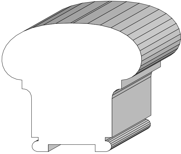
BA 852 2-5/16" x 2-1/8"
