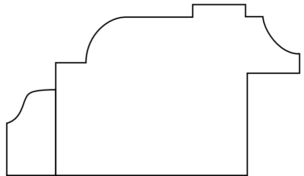
BA 693A 1-3/4" x 2-1/2" BA 693C 1/2 x 7/8"
