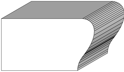
BA 590 1-1/8" x 2"
