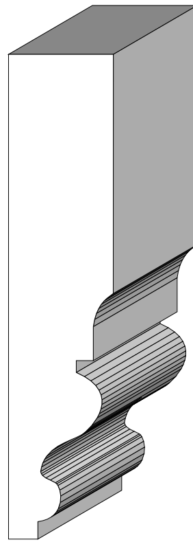
BA 581 13/16" x 3-11/16"
