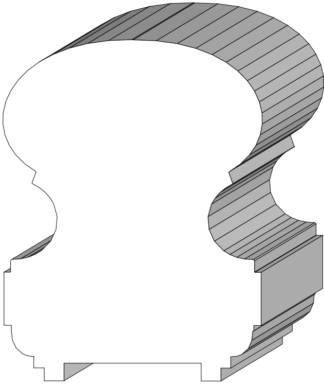
BA 513 2-5/8" x 3-1/2"
