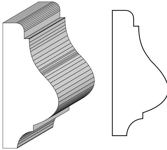
BA 150 1" x 2-1/4"
