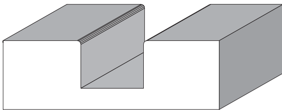
BA 358 1/2" x 5/8" Dado
