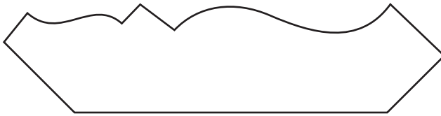
BA 2066 13/16" x 3-1/4"
