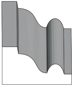
BA 1638 5/8" x 1-3/16"
